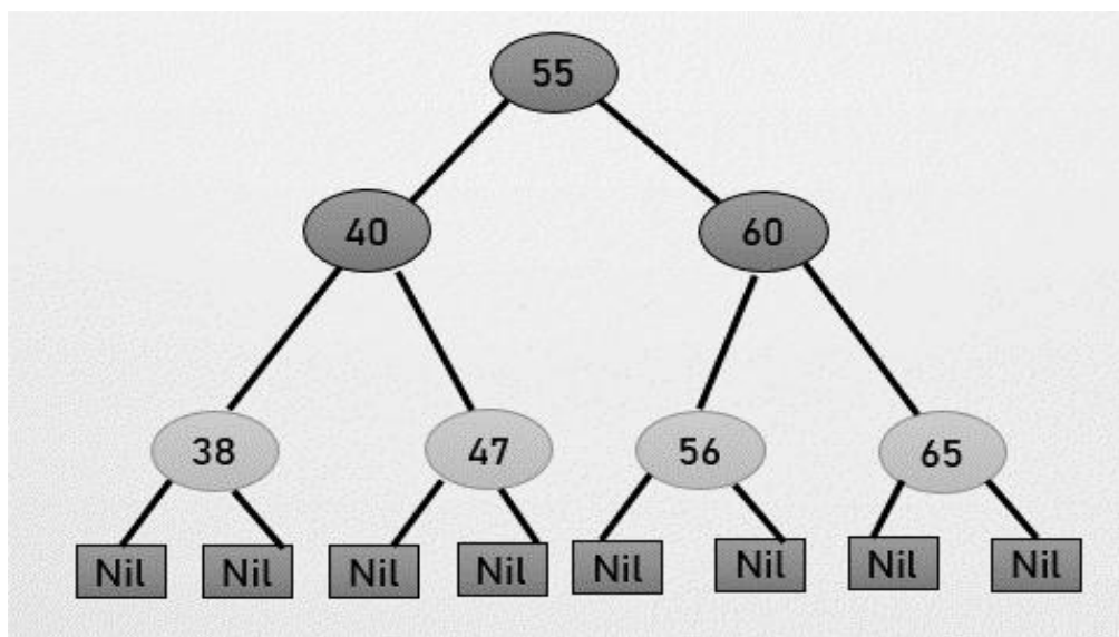
Red-black tree
