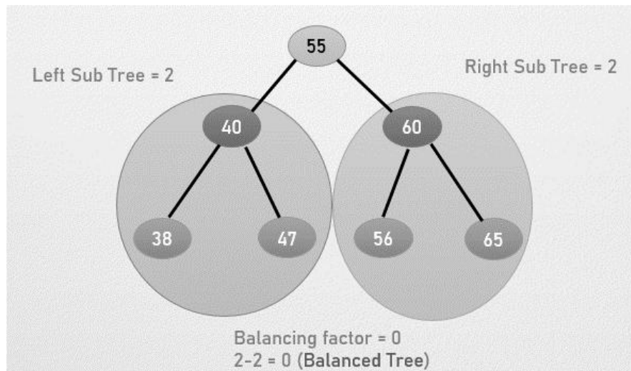
Balanced Tree
